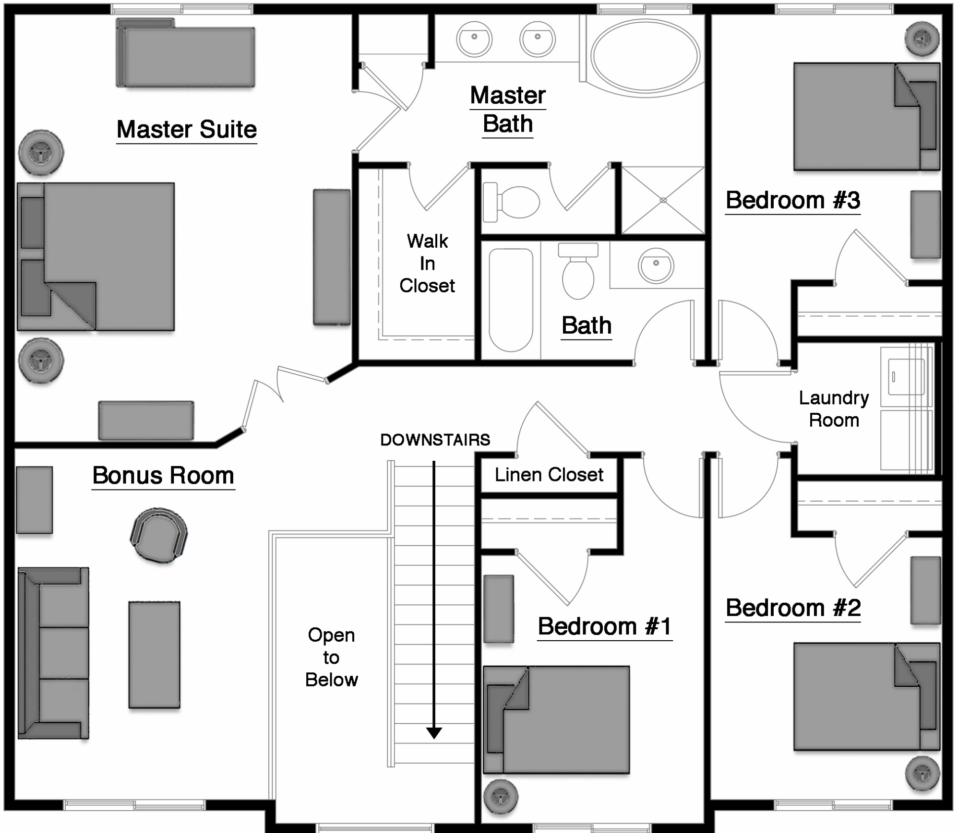
Upper Floor
